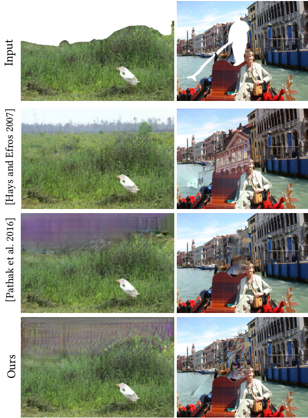
Fig. 13. Failure cases from the dataset of [Hays and Efros 2007]. For the comparison, we have retrained the model of [Pathak et al. 2016] on the Places2 dataset for arbitrary regions. The image on the left corresponds to a case of image extrapolation, i.e. , the inpainting mask lies on the boundary of the image. Out of the 51 images in this dataset, 32 have masks that correspond to image extrapolation. Additional results can be found in the supplemental materials.
